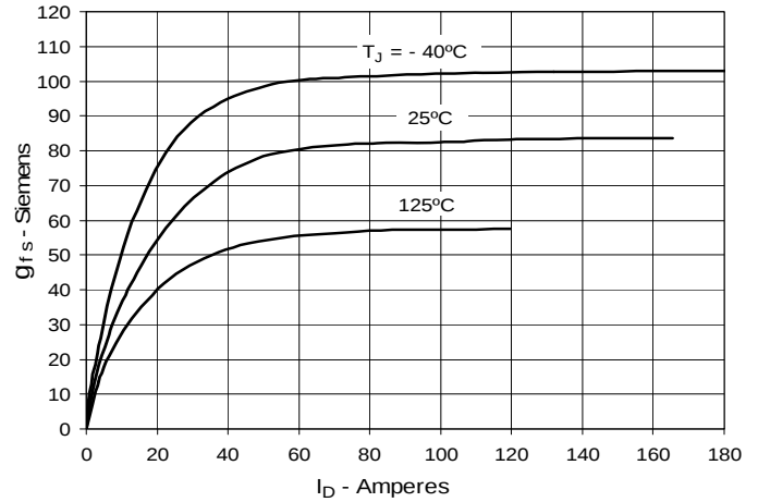
Fig. 8. Transconductance
