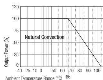
RP15-4805SAW With Heat Sink
