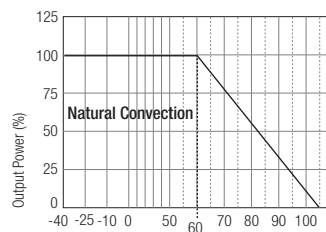
RP15-4805SAW With Heat Sink
