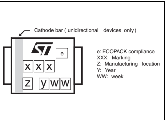
Figure 21. Marking layout (1)
