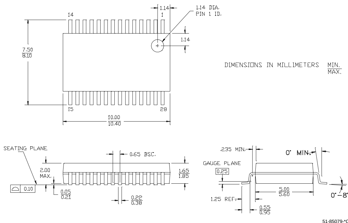
Figure 12-2. 28-Lead Shrunk Small Outline Package
