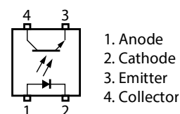
PIN CONNECTION (Top View)
