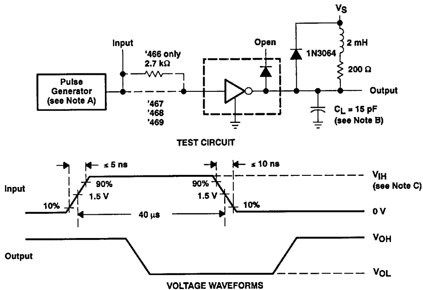
Figure 10. Latch-Up Test Circuit and Voltage Waveforms
