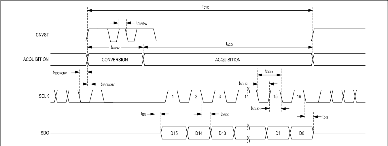
Figure 6. \overline{\text{CS}} Mode 3-Wire, No-Busy Indicator Serial Interface Timing (SDI High)
