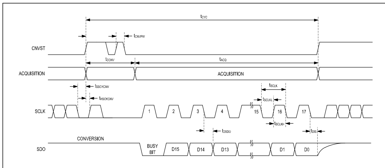
Figure 8. \overline{CS} Mode 3-Wire with Busy Indicator Serial Interface Timing (SDI High)
