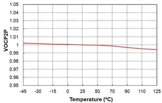
Figure 49. V OCP2P vs. Temperature
