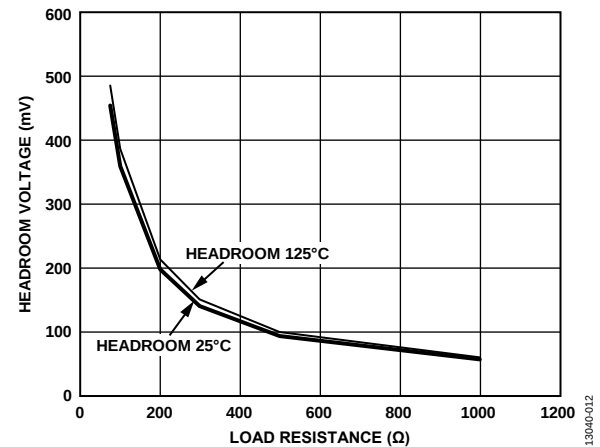
Figure 12. Typical Headroom Voltage vs. Load Resistance for VDAC4, AV_{DD} = 3\text{ V} ; Headroom = AV_{DD} - V_{DAC} Output Voltage
