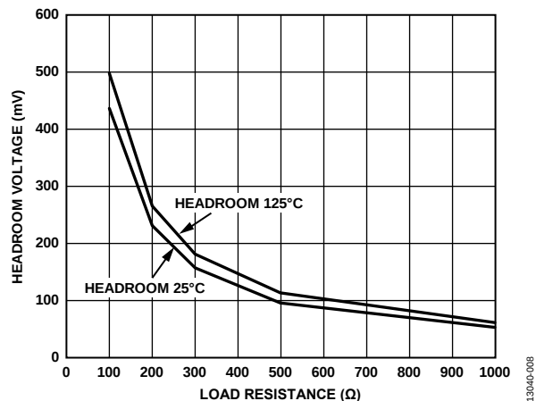
Figure 8. Typical Headroom Voltage vs. Load Resistance for VDAC7, V_{DACV_{DD}} = 3\text{ V} ; Headroom = V_{DACV_{DD}} - V_{DAC} Output Voltage
