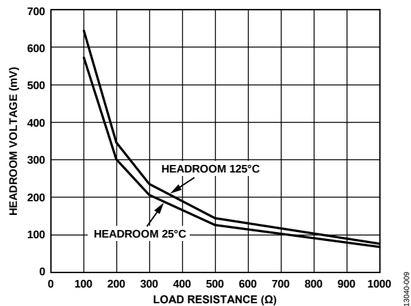
Figure 9. Typical Headroom Voltage vs. Load Resistance for VDAC7, V_{DACV_{DD}} = 5\text{ V} ; Headroom = V_{DACV_{DD}} - V_{DAC} Output Voltage
