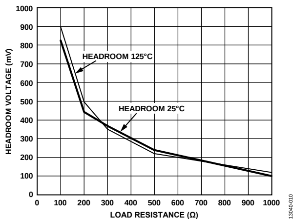
Figure 10. Typical Headroom Voltage vs. Load Resistance for VDAC2, AV_{NEG} = -5\text{ V} ; Headroom = AV_{NEG} - V_{DAC} Output Voltage
