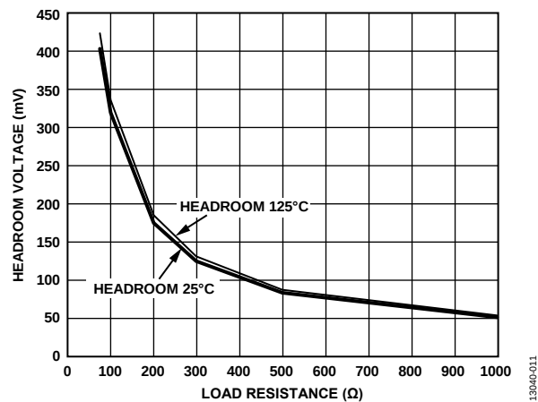
Figure 11. Typical Headroom Voltage vs. Load Resistance for VDAC0, AV_{DD} = 3\text{ V} ; Headroom = AV_{DD} - V_{DAC} Output Voltage
