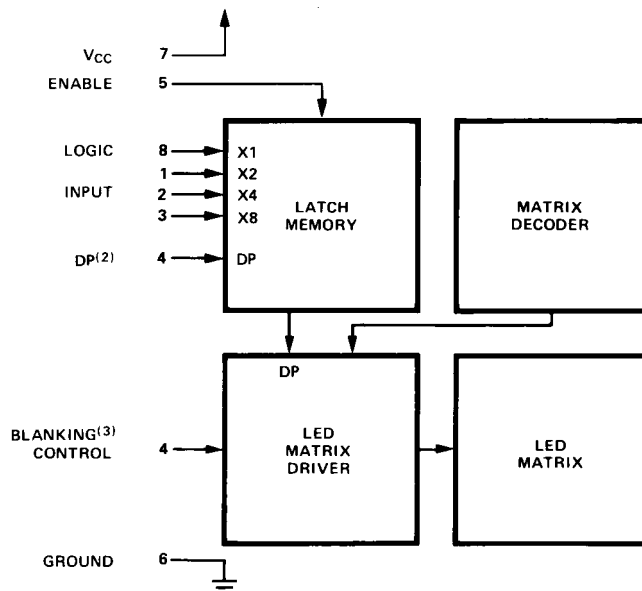
Figure 2. Block Diagram.
