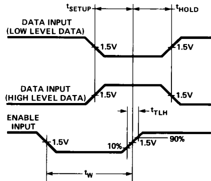
Figure 1. Timing Diagram.
