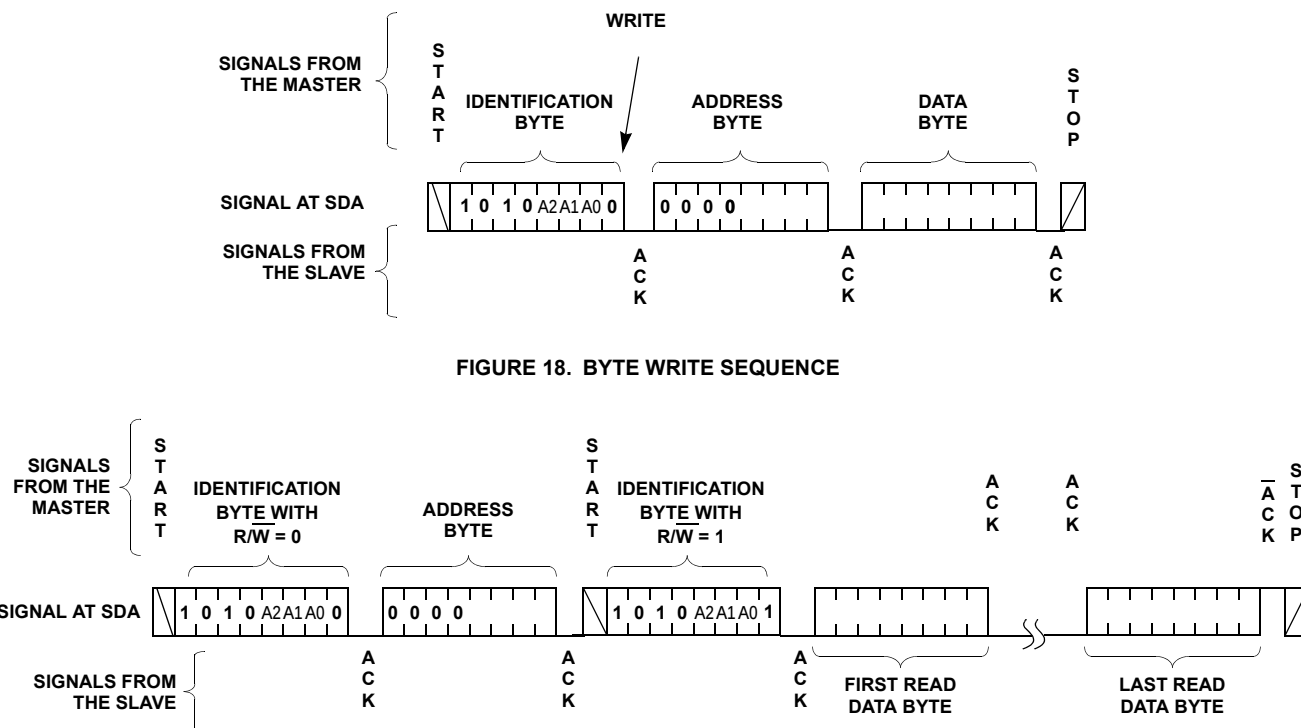
FIGURE 19. READ SEQUENCE
