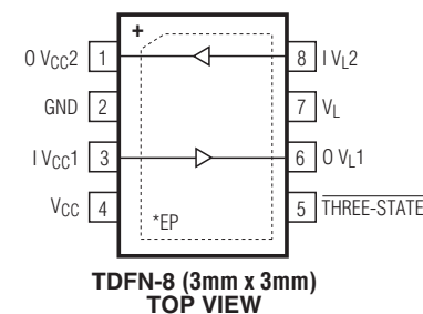
TDFN-8 (3mm x 3mm) TOP VIEW
