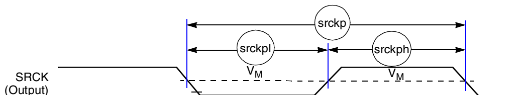
Figure 81. SPDIF Timing Diagram
