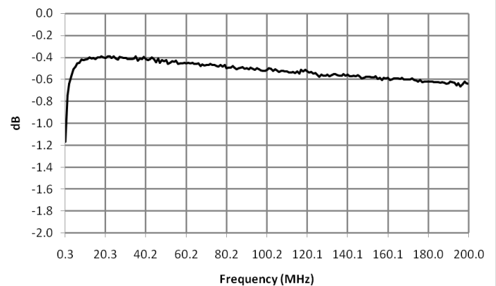
MABAES0060insertion_loss_pin_4_1
