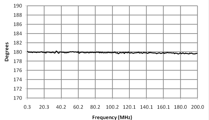
MABAES0060phase_balance
