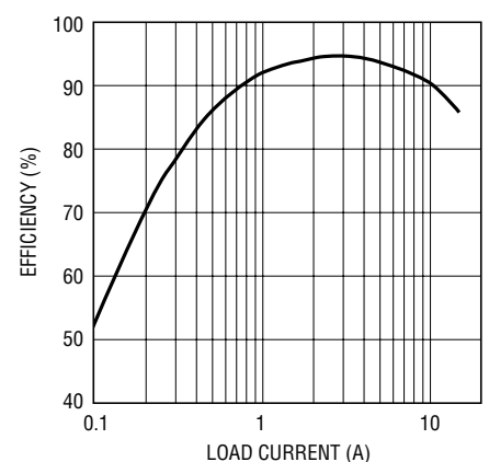
LTC1649 Efficiency
