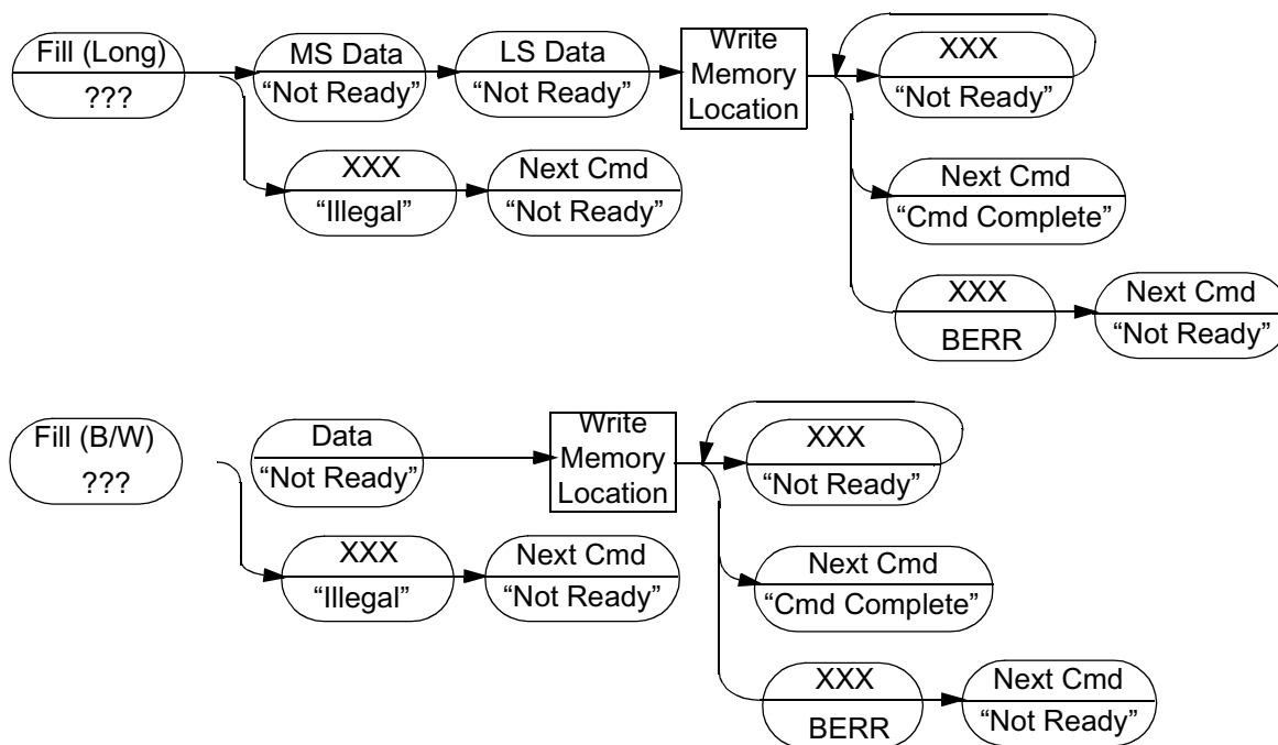
Figure 19-14 Fill Memory Block Command Sequence
