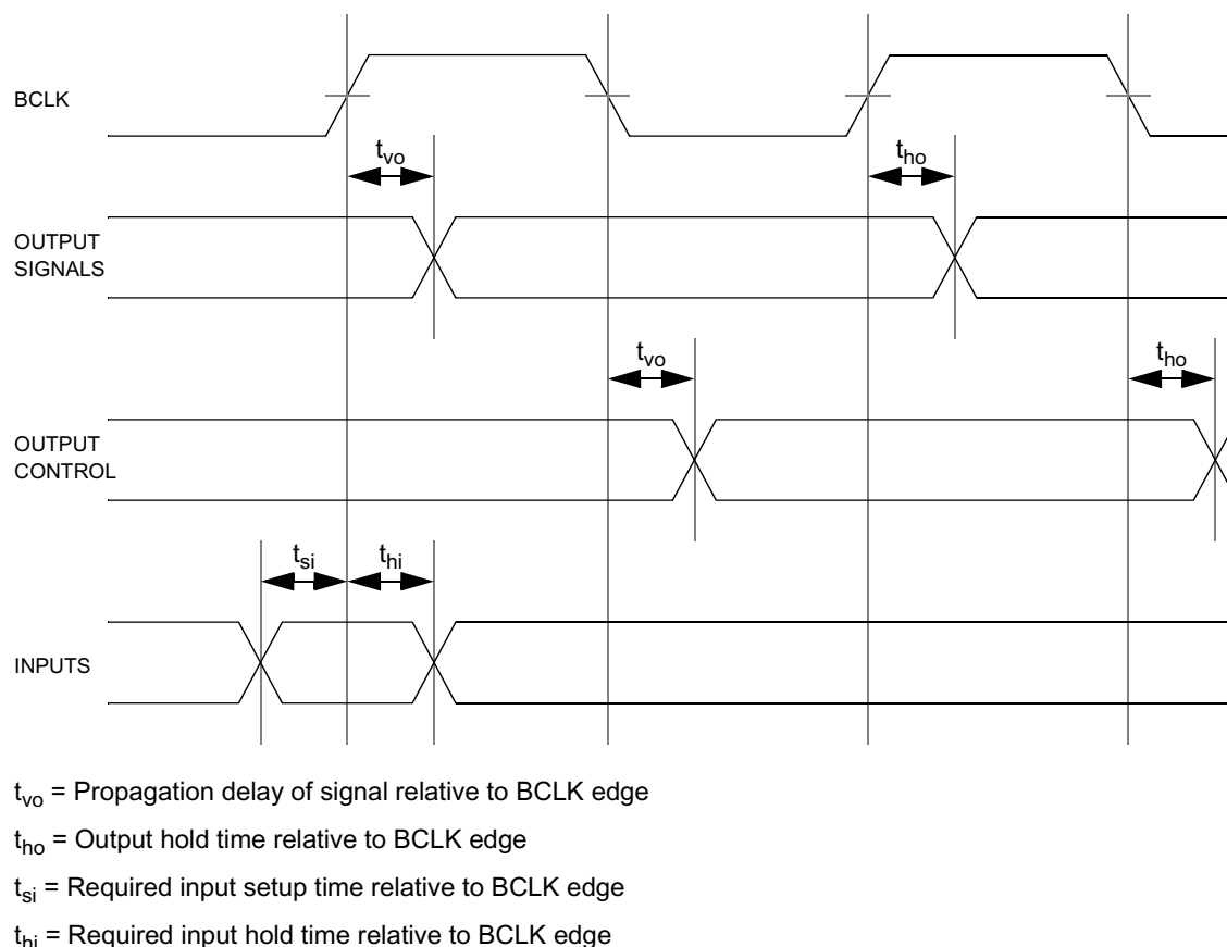
Figure 8-2 Signal Relationship to BCLK for Non-DRAM Access
