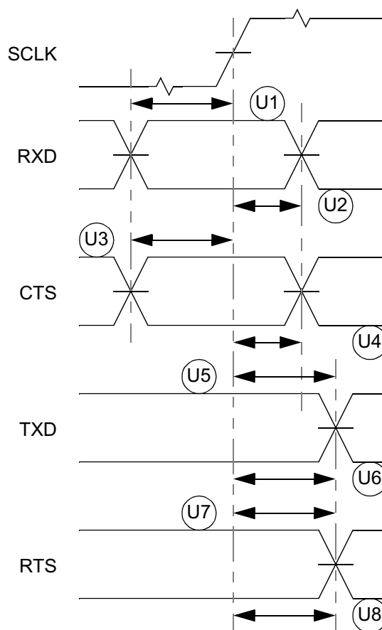
Figure 21-11 UART Timing Definition
