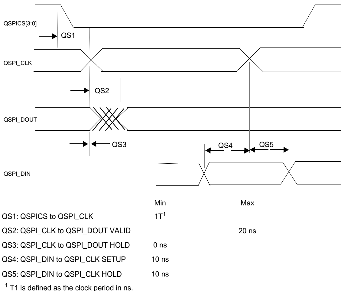
Figure 16-11 QSPI Timing
