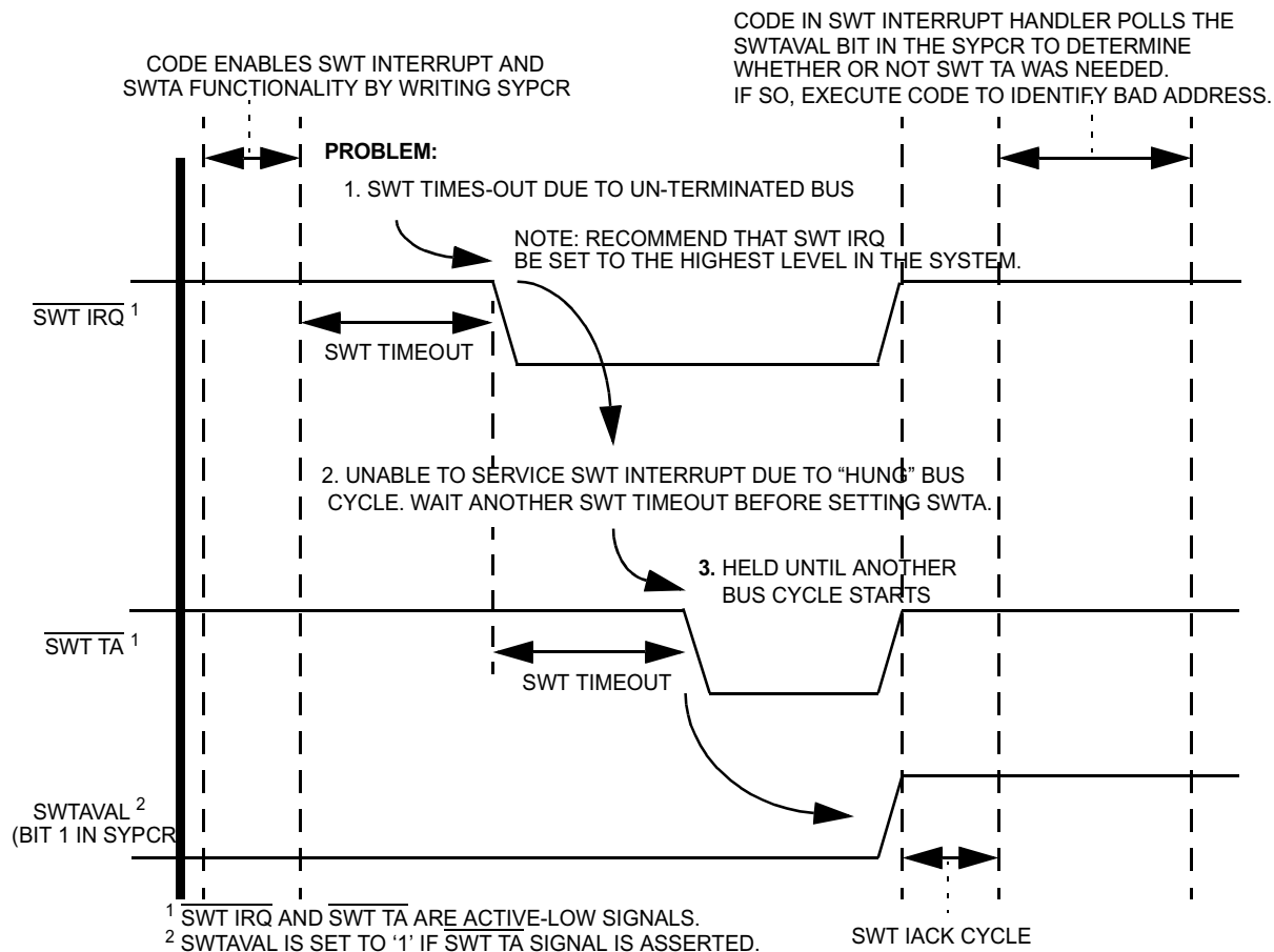
Figure 9-1 MCF5249 Underterminated Access Recovery
