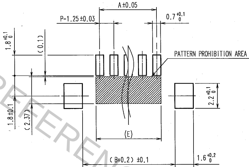
RECOMMENDED PATTERN
