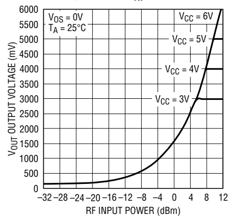
V_{OUT} vs RF Input Power and V_{CC} Supply Voltage, f_{RF} = 2GHz
