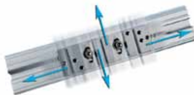
The brackets are designed to allow for movement along two axis.
