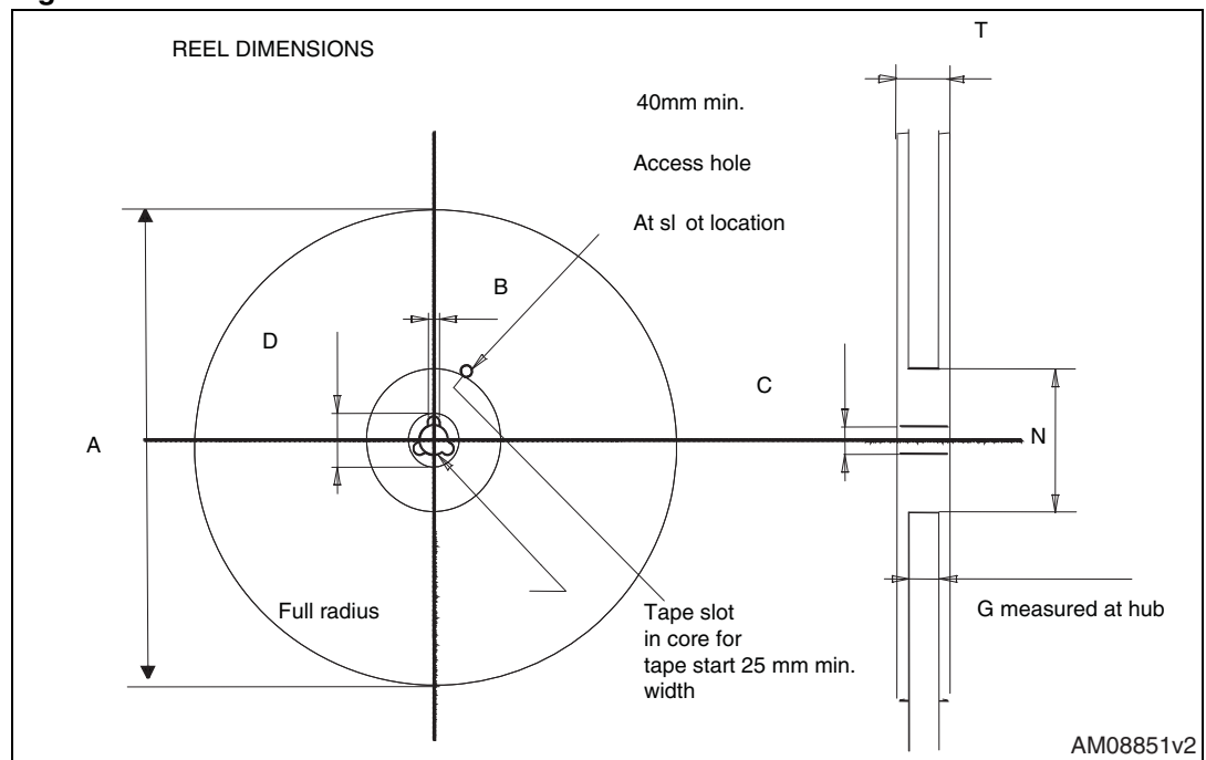
Figure 25. Reel
