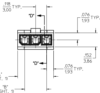
.079 REF. 2.00 TERMINAL INSERTION DEPTH
