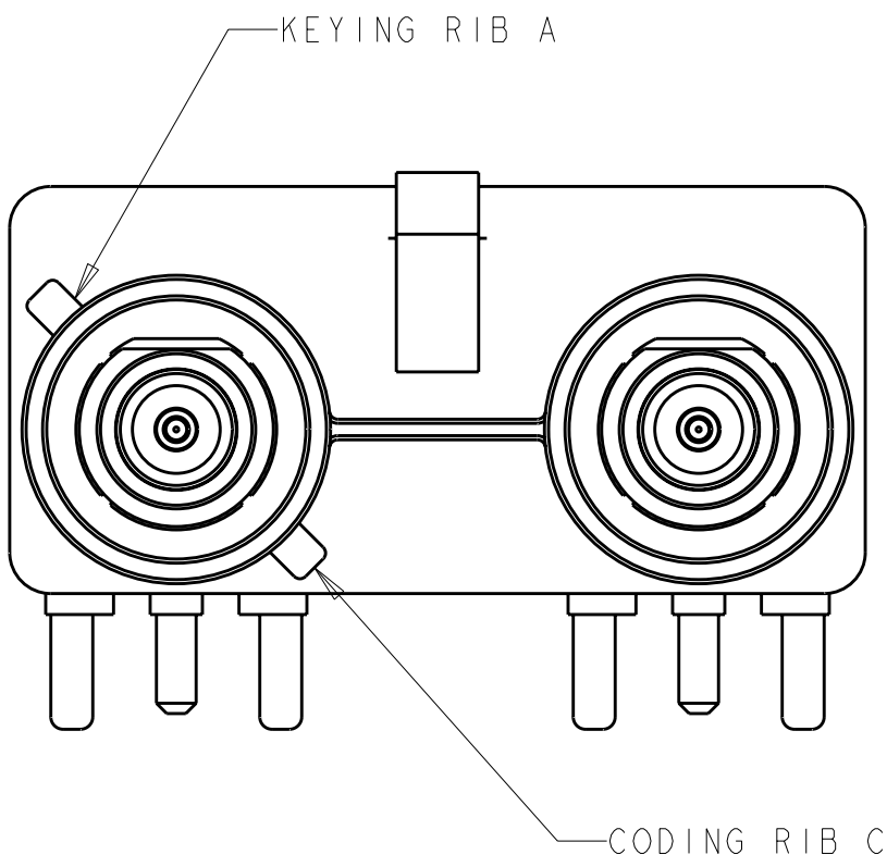
DETAIL S
