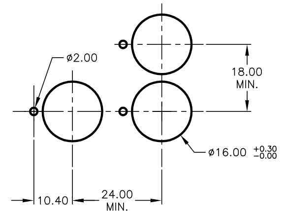
RECOMMENDED PANEL MOUNTING SCALE 1:1
