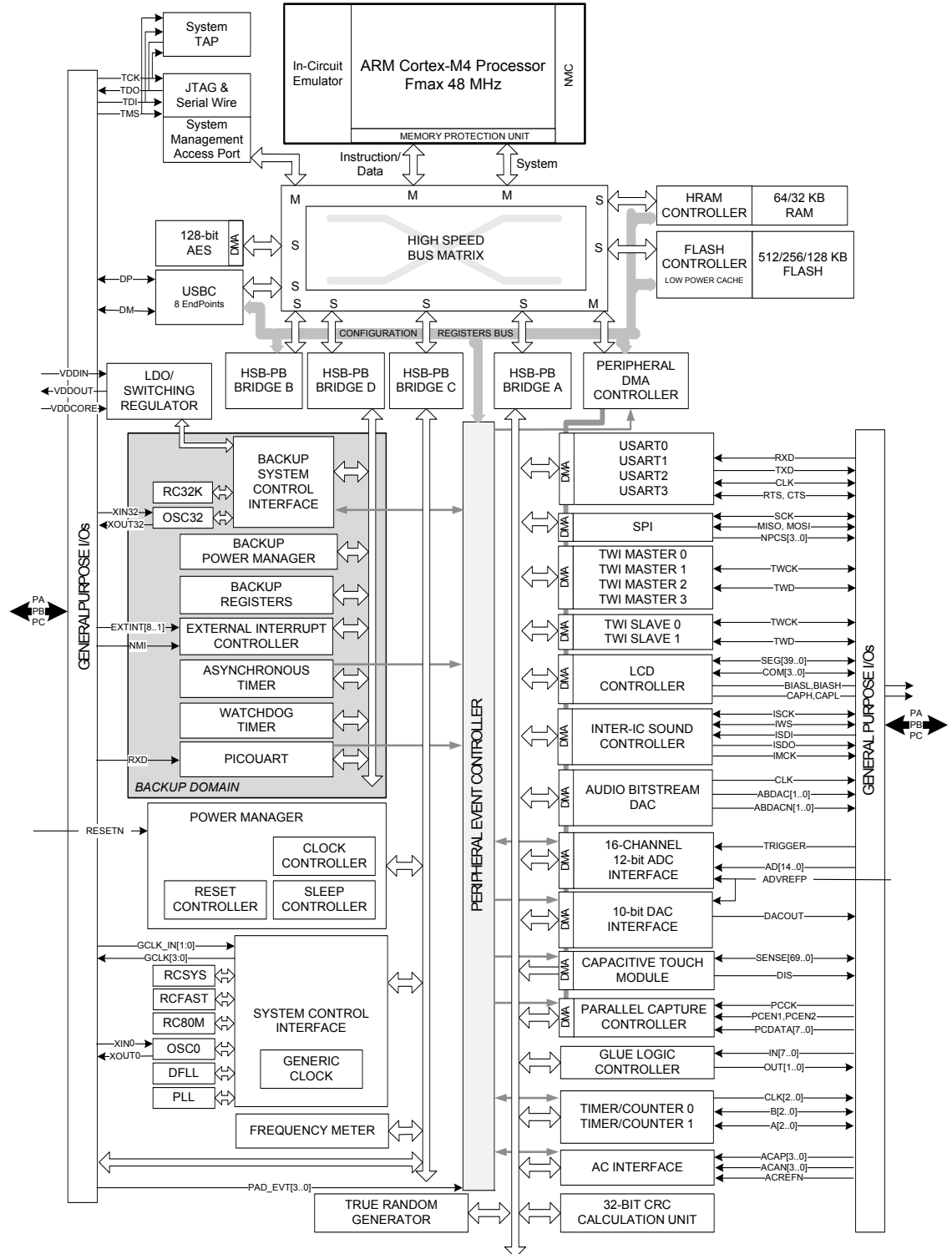
Figure 2-1. Block Diagram
