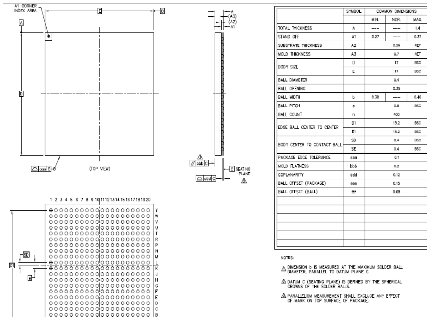
Figure 22. KSZ8692PB-S 400-Pin PBGA (17X17X1.4 MM)
