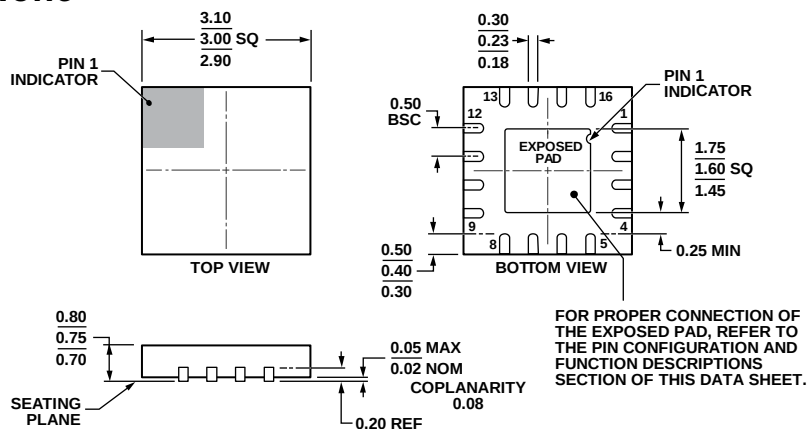
Figure 55. 16-Lead Lead Frame Chip Scale Package [LFCSP_WQ] 3 mm × 3 mm Body, Very Very Thin Quad (CP-16-22) Dimensions shown in millimeters
