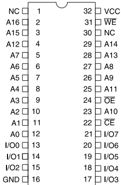
PDIP Top View
