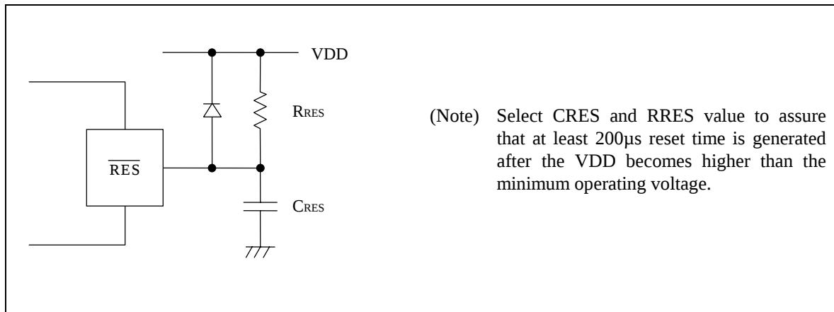
Figure 5 Reset circuit
