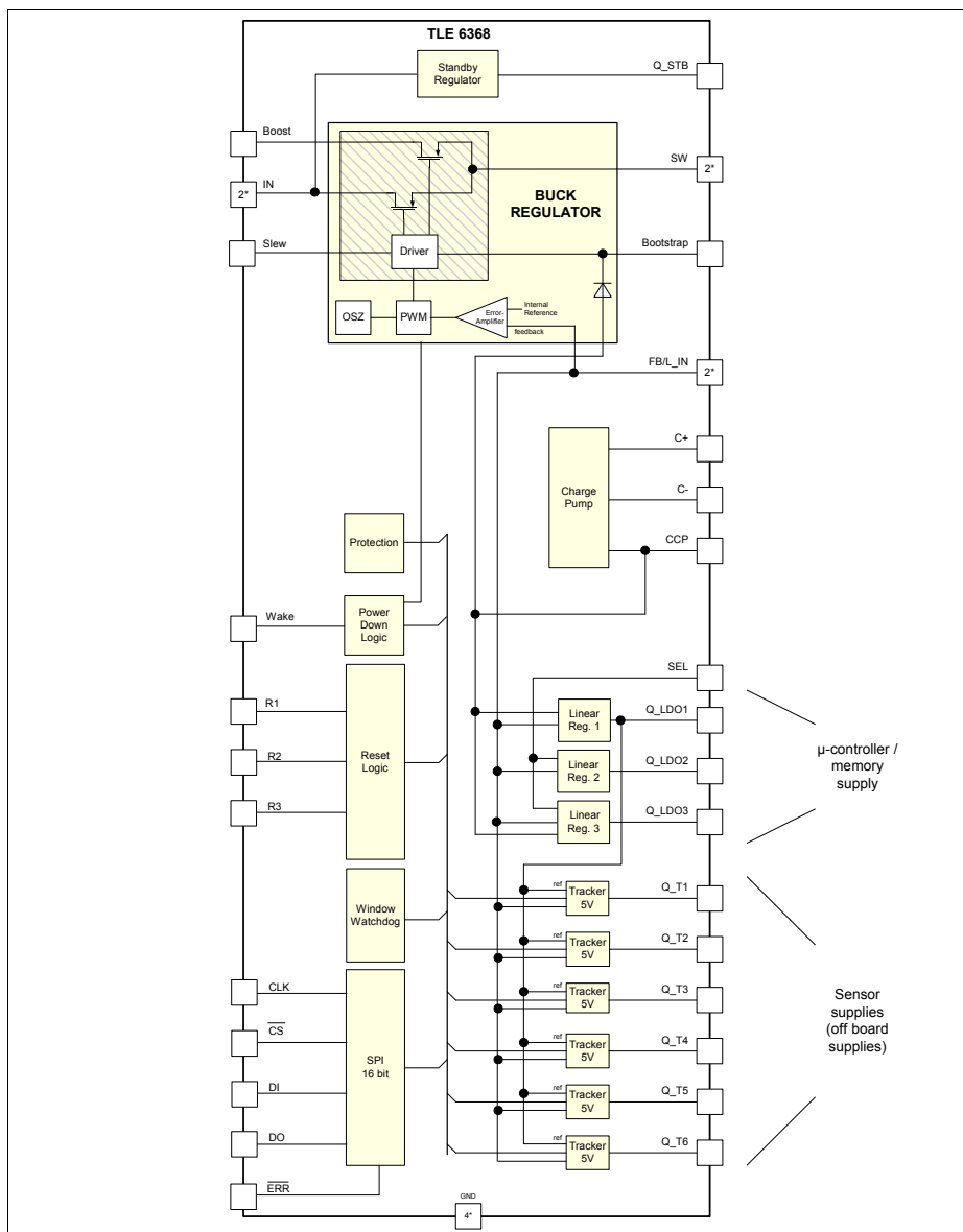
Figure 2 Block Diagram
