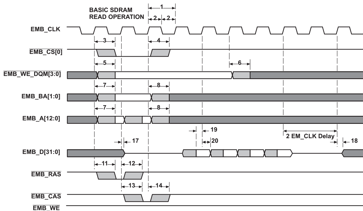
Figure 5-20. EMIFB Basic SDRAM Read Operation
