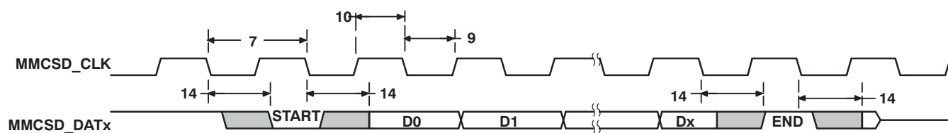
Figure 5-23. MMC/SD Host Write Timing
