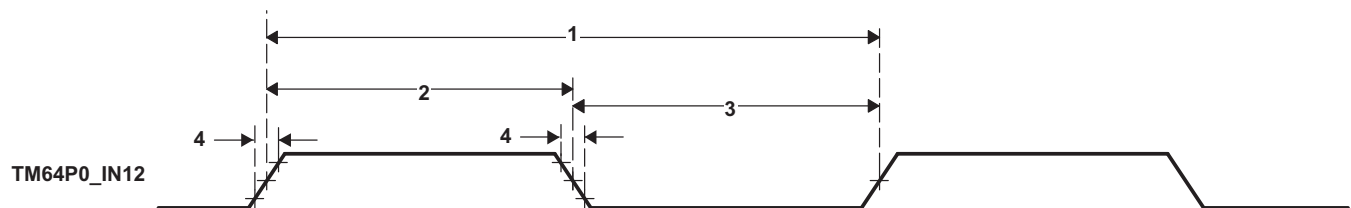
Figure 5-42. Timer Timing
