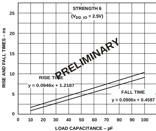
Figure 40. Typical Output Rise and Fall Time (10%–90%, V_{DD\_IO} = 2.5V ) vs. Load Capacitance at Strength 6
