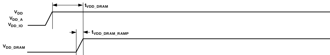
Figure 8. Power-Up Timing
