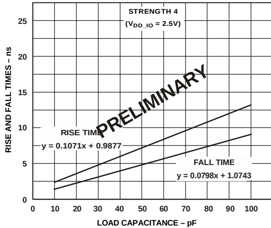
Figure 38. Typical Output Rise and Fall Time (10%–90%, V_{DD\_IO} = 2.5V ) vs. Load Capacitance at Strength 4
