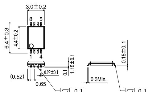
SSOP-B8
