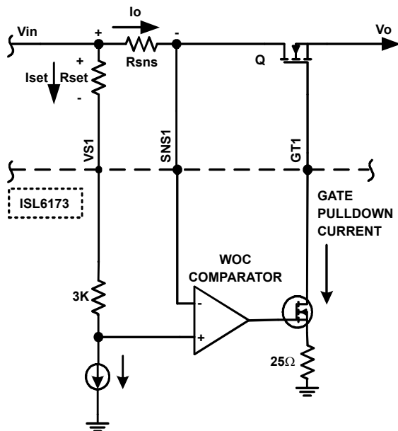
FIGURE 14. WOC OPERATION
