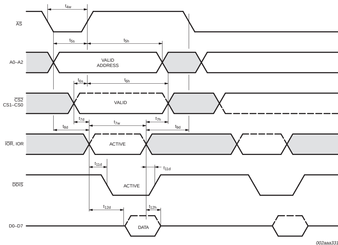
Fig 11. General read timing when using \overline{\text{AS}} signal.
