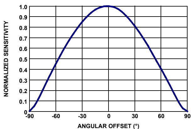
FIGURE 8. ANGULAR SENSITIVITY
