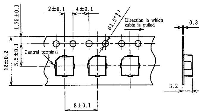
Emboss tapping specifications
