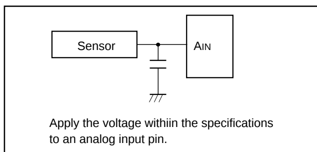
Fig. 53 Analog input external circuit example-1
