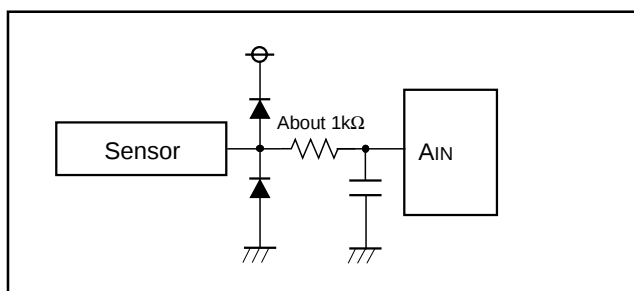
Fig. 54 Analog input external circuit example-2
