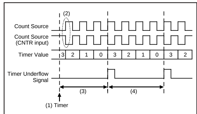
Fig. 48 Timer count start timing and count time when operation starts (T1, T2)
