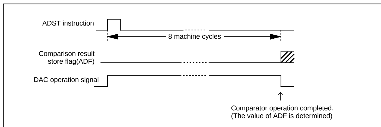
Fig. 31 Comparator operation timing chart
