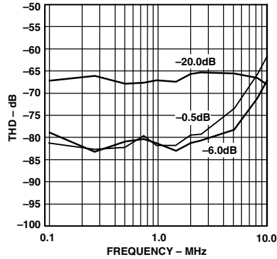
TPC 14. THD vs. Input Frequency (Input Span = 2.0 V p-p, V_{CM} = 2.5 \text{ V} )
