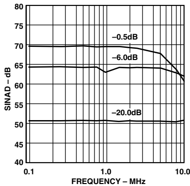
TPC 13. SINAD vs. Input Frequency (Input Span = 2.0 V p-p, V_{CM} = 2.5 \text{ V} )
