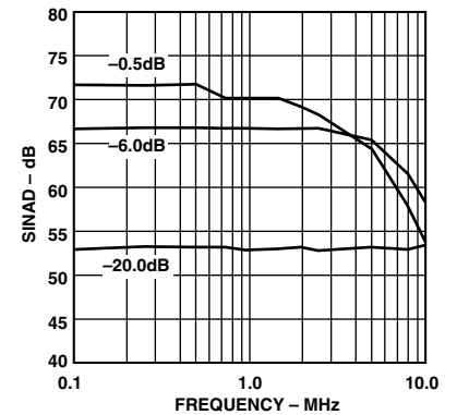
TPC 15. SINAD vs. Input Frequency (Input Span = 5.0 V p-p, V_{CM} = 2.5 \text{ V} )
