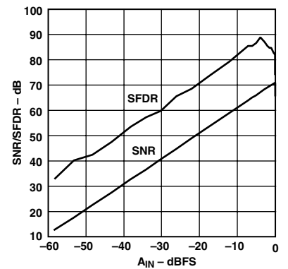
TPC 18. SNR/SFDR vs. A_{IN} (Input Amplitude) ( f_{IN} = 1.5 \text{ MHz} , Input Span = 2 V p-p, V_{CM} = 2.5 \text{ V} )
