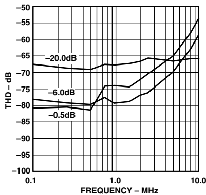
TPC 16. THD vs. Input Frequency (Input Span = 5.0 V p-p, V_{CM} = 2.5 \text{ V} )
