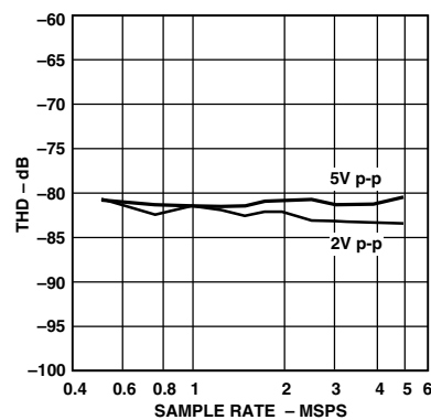
TPC 17. THD vs. Sample Rate ( A_{IN} = -0.5 \text{ dB} , f_{IN} = 500 \text{ kHz} , V_{CM} = 2.5 \text{ V} )
