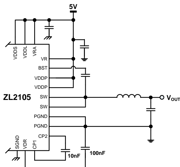
Figure 11. Powering the Low-side Driver When V_{DDDS} \leq 5.5 V
