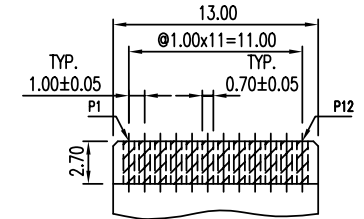
DETAIL 'A' (CONNECTOR SIDE OF FPC) (DOWNSIDE CONTACT)
