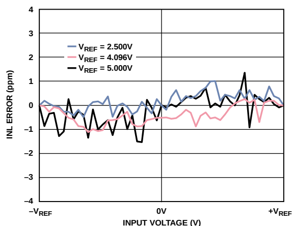
Figure 42. INL Error vs. Input Voltage for Various Voltage Reference ( V_{REF} ) Levels, Eco Mode
