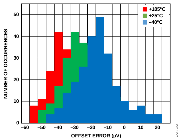
Figure 45. Offset Error Distribution, DCLK = 24 MHz
