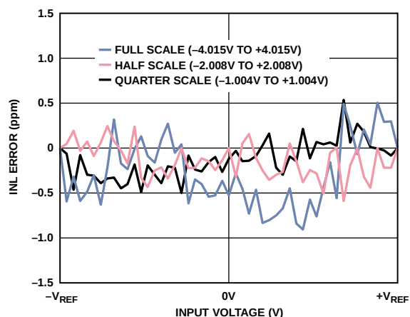
Figure 43. INL Error vs. Input Voltage, Full-Scale, Half-Scale, and Quarter-Scale Inputs
