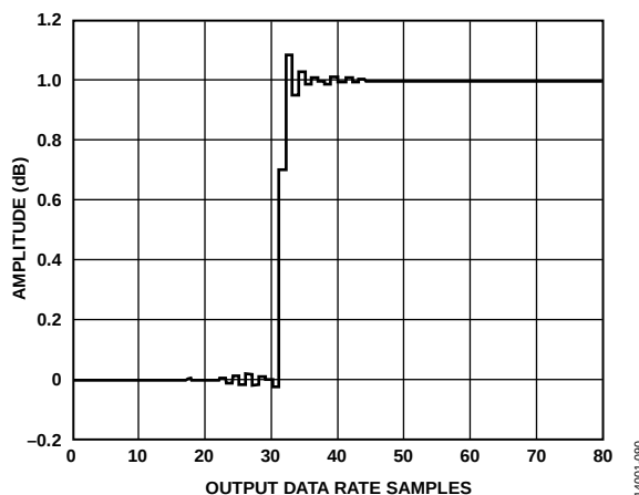
Figure 90. Wideband Filter Step Response
