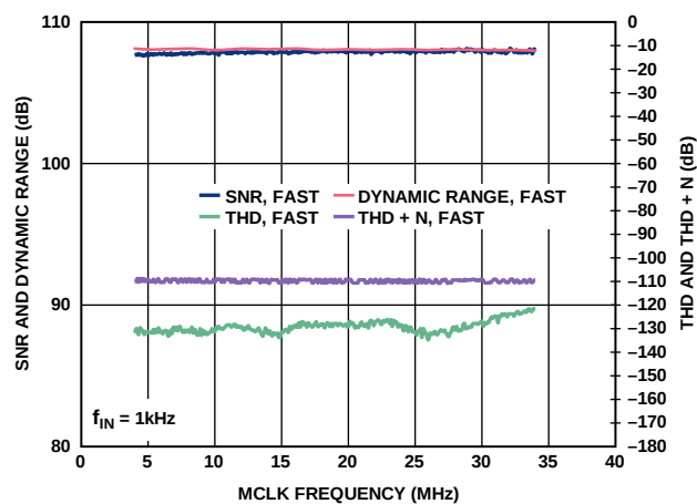
Figure 34. SNR, Dynamic Range, THD, and THD + N vs. MCLK Frequency
