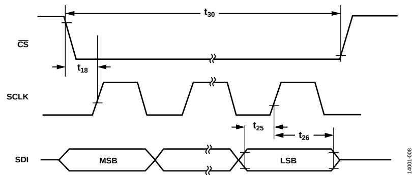
Figure 8. SPI Serial Write Timing Diagram
