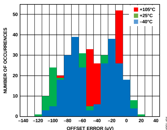
Figure 46. Offset Error Distribution, DCLK = 32 MHz
