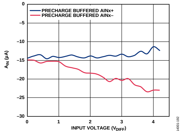
Figure 86. Analog Input Current ( A_{IN} ) vs. Input Voltage, Analog Input Precharge Buffer On, V_{CM} = 2.5 V, f_{MOD} = 8.192 MHz
