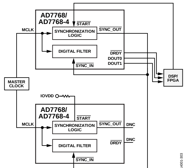
Figure 105. Synchronizing Multiple AD7768/AD7768-4 Devices Using SYNC OUT
