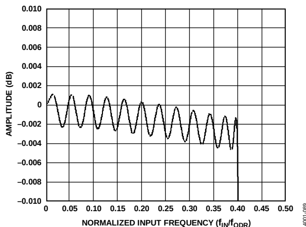
Figure 89. Wideband Filter Pass-Band Ripple
