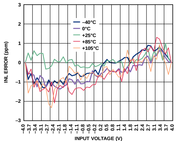
Figure 44. INL Error vs. Input Voltage for Various Temperatures, Fast Mode
