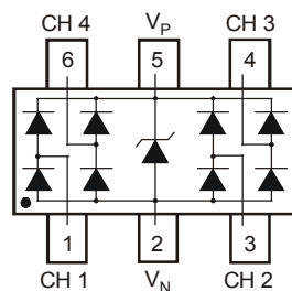
Device Schematic
