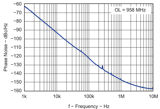
Figure 50. Open Loop VCO Phase Noise
