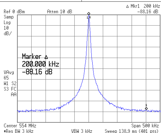
Figure 82. Divide-By-4 Output: PFD Frequency Spurs
