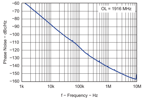
Figure 48. Open Loop VCO Phase Noise
