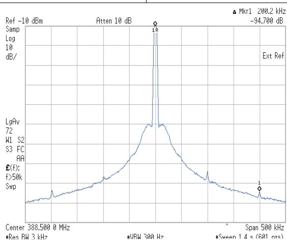
Figure 19. Divide-By-4 Output: PFD Frequency Spurs
