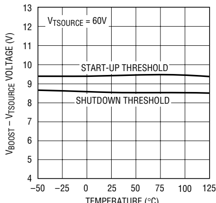
Undervoltage Lockout (VBOOST)
