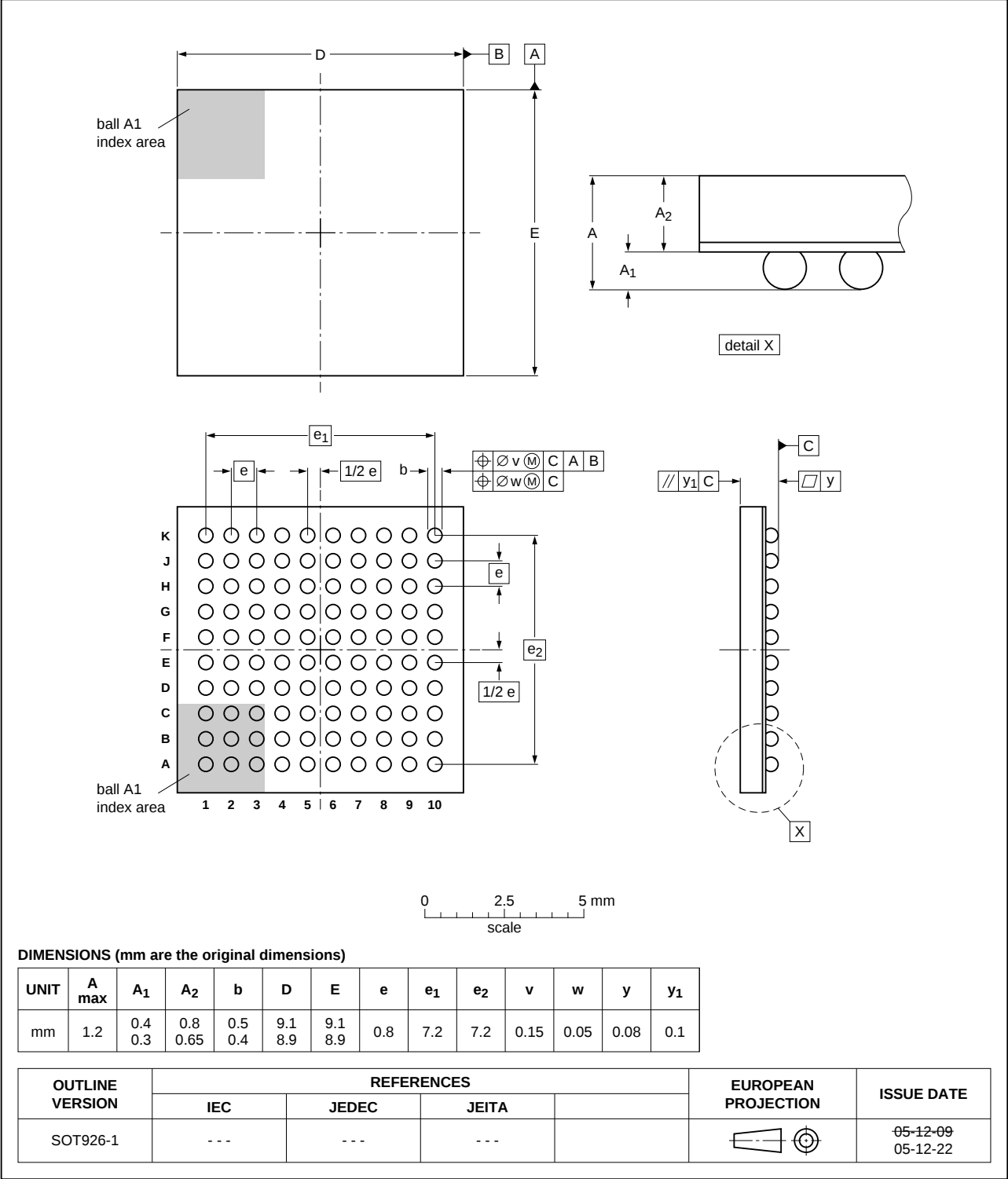
Fig 46. Package outline of the TFBGA100 package
