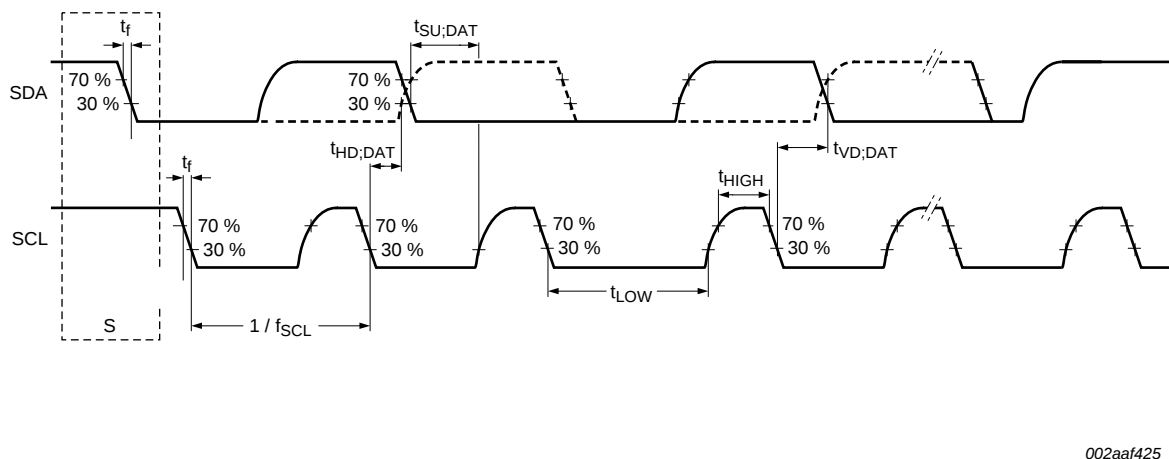
Fig 25. I 2 C-bus pins clock timing
