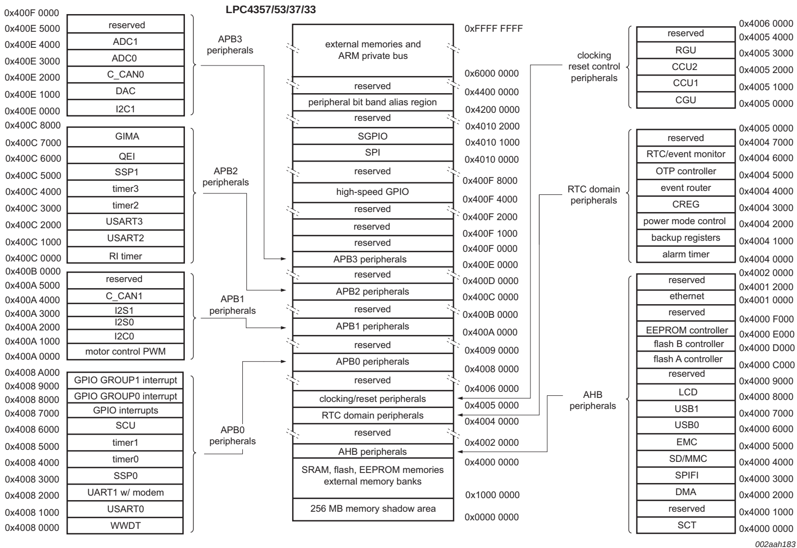
Fig 9. LPC4357/53/37/33 Memory mapping (peripherals)
