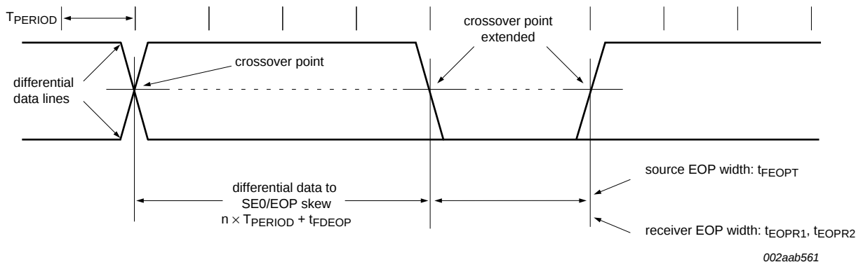
Fig 33. Differential data-to-EOP transition skew and EOP width
