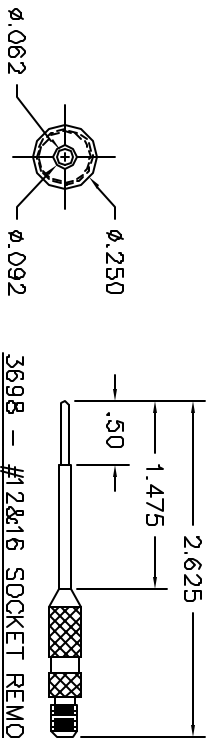
8251 - #8 SOCKET REMOVAL
