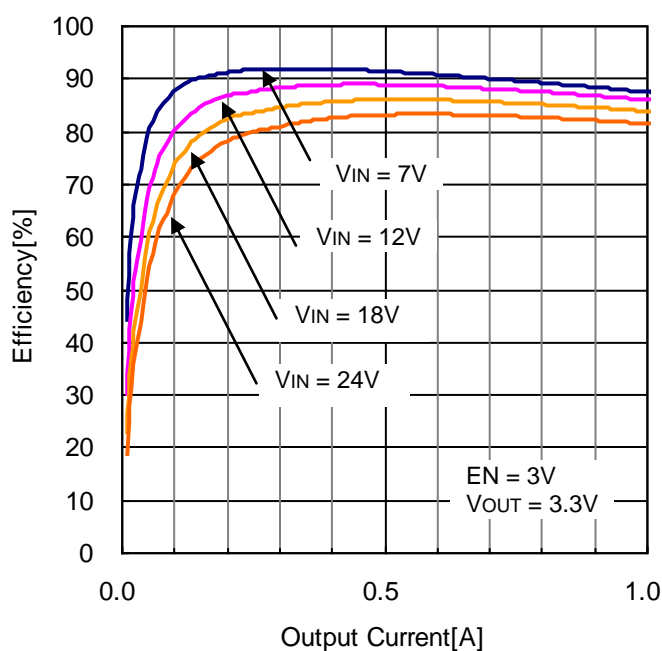
Figure 18. Efficiency vs Output Current (VOUT = 3.3V, L=10μH)
