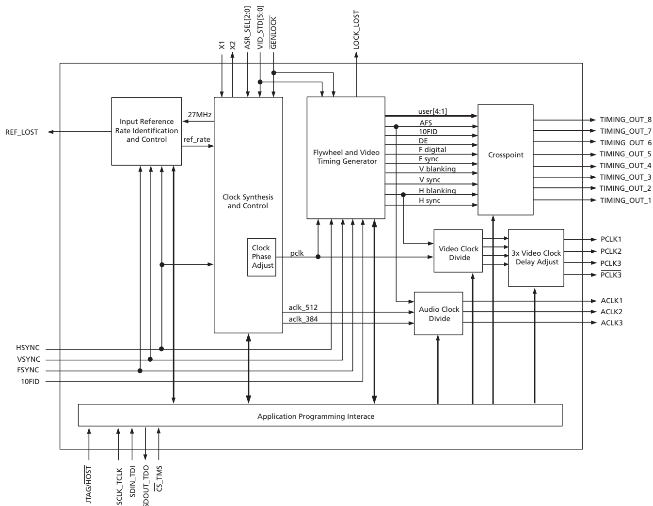
GS4901B Functional Block Diagram
