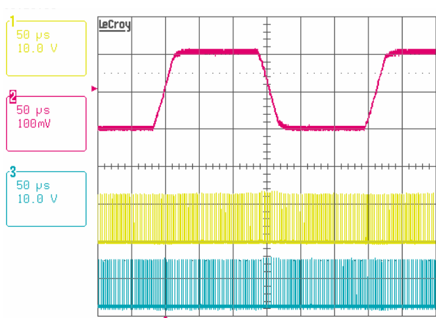
FIGURE 47. 2-PHASE CPU MODE VID ON THE FLY, 1.075V/0.875V, 2-PHASE CONFIGURATION, PSI# = 1, DPRSLPVR = 0, Ch1: PHASE1, Ch2: V_O , Ch3: PHASE2
