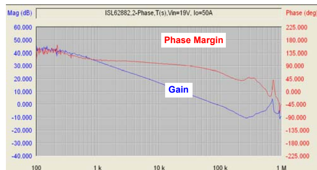
FIGURE 51. 2-PHASE CPU MODE REFERENCE DESIGN LOOP GAIN T2(s) MEASUREMENT RESULT
