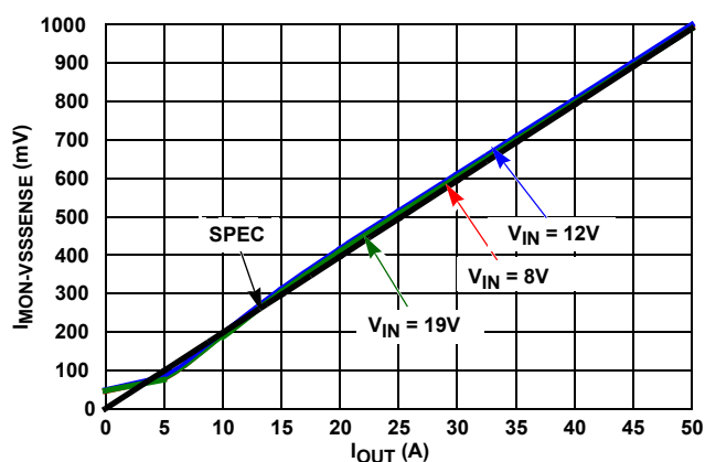
FIGURE 52. IMON, V_{ID} = 1.075
