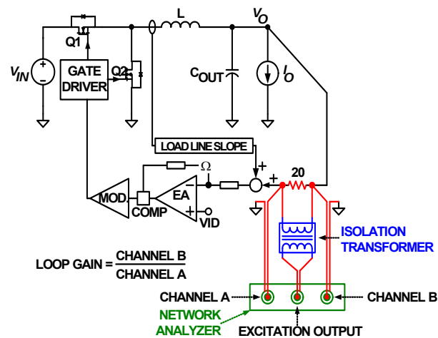
FIGURE 26. LOOP GAIN T2(s) MEASUREMENT SET-UP
