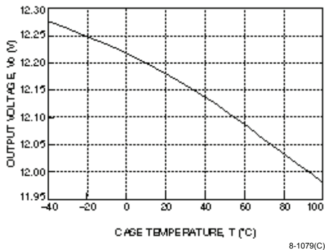
Figure 3. CC025 Triple-Output-Series Typical Output Voltage Variation of 12 V Output Over Ambient Temperature Range
