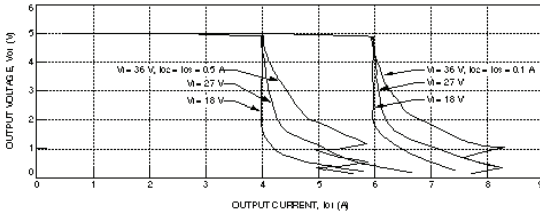
Figure 9. CC025ABK-M Typical 5 V Output Characteristics
