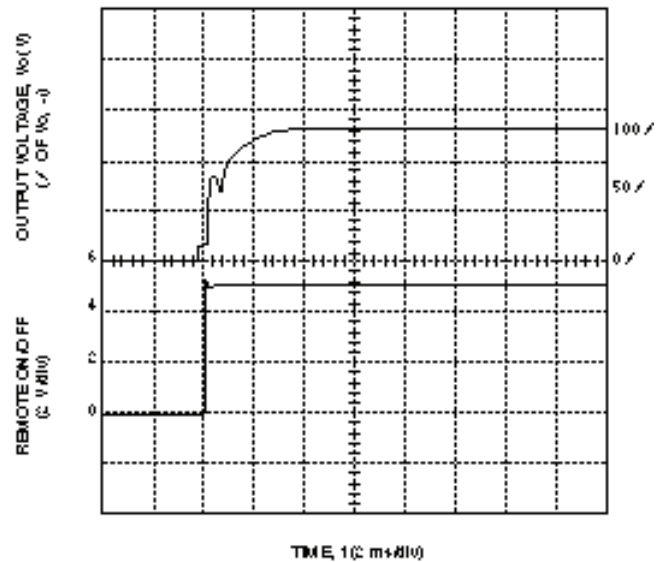
Figure 17. CC025 Triple-Output-Series Typical Output Voltage Start-Up when Signal Applied to Remote On/Off
