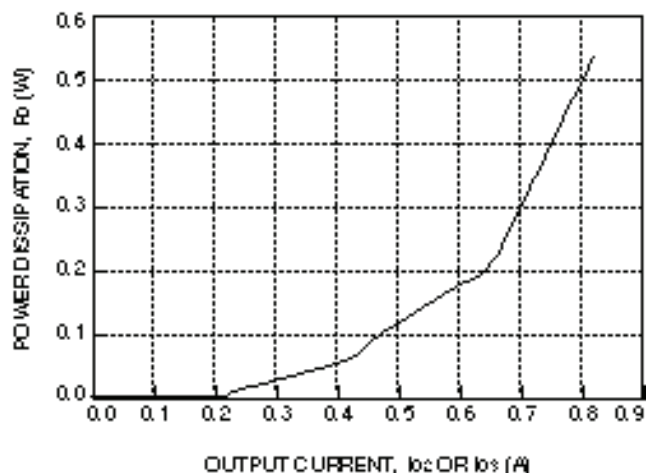
Figure 27. CC025ACL-M Losses Associated with ±15 V Output, Ps2/Ps3
