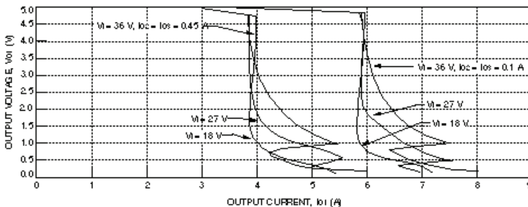
Figure 11. CC025ACL-M Typical 5 V Output Characteristics
