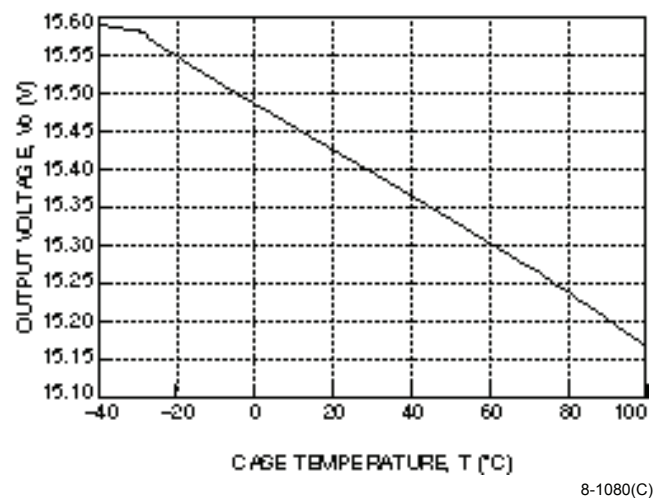
Figure 4. CC025 Triple-Output-Series Typical Output Voltage Variation of 15 V Output Over Ambient Temperature Range
