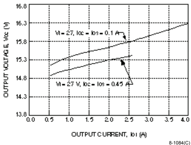
Figure 8. CC025ACL-M Typical Cross Regulation with Respect to I_{o1}
