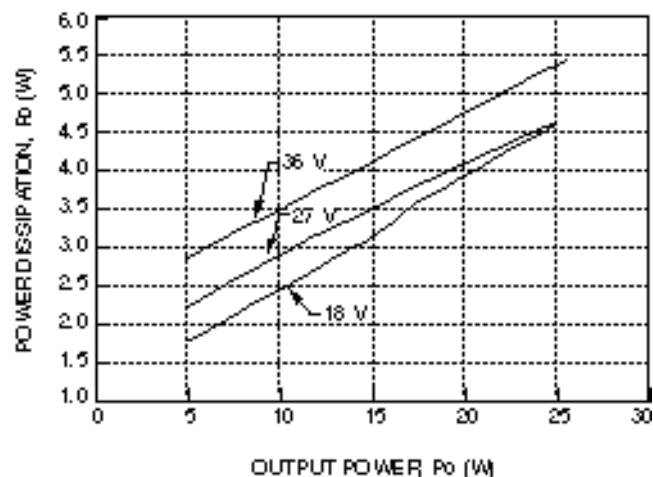
Figure 23. CC025ABK-M Fixed Losses, P_p
