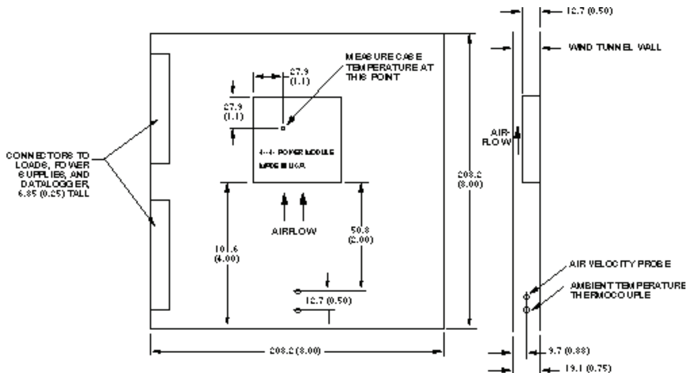
Figure 22. Thermal Test Setup
