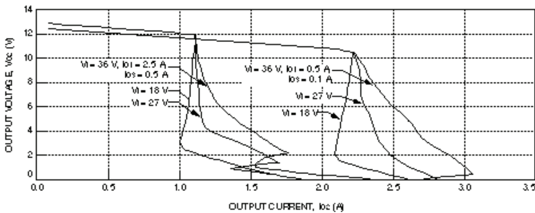
Figure 10. CC025ABK-M Typical 12 V Output Characteristics
