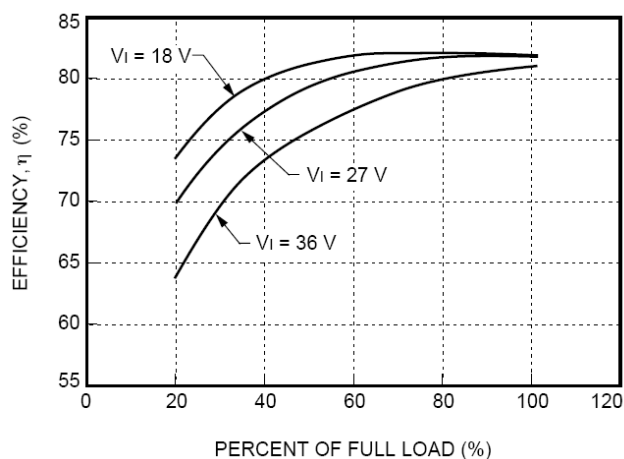
Figure 13. CC025ABK-M Typical Converter Efficiency
