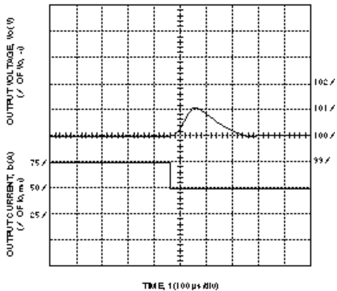
Figure 15. CC025 Triple-Output-Series Typical Output Voltage for a Step Load Change from 75% to 50% of Full Load on Output 1
