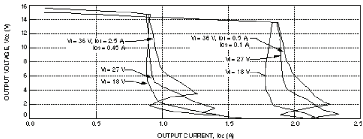
Figure 12. CC025ACL-M Typical 15 V Output Characteristics
