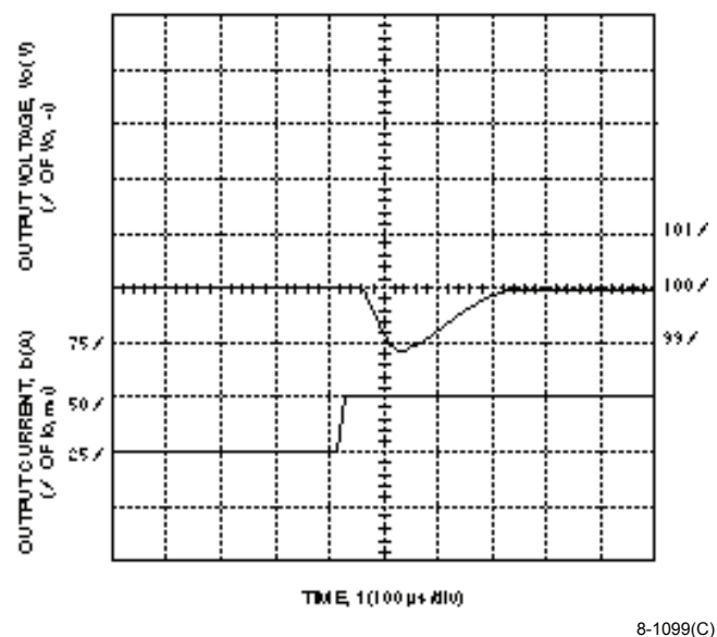
Figure 16. CC025 Triple-Output-Series Typical Output Voltage for a Step Load Change from 25% to 50% of Full Load on Output 1
