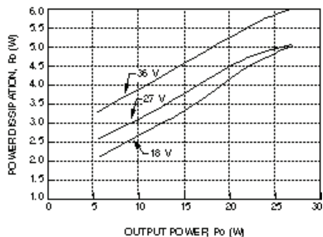
Figure 24. CC025ACL-M Fixed Losses, P_p
