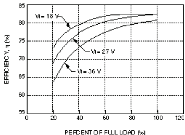
Figure 14. CC025ACL-M Typical Converter Efficiency
