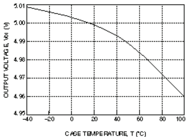
Figure 2. CC025 Triple-Output-Series Typical Output Voltage Variation of 5 V Output Over Ambient Temperature Range
