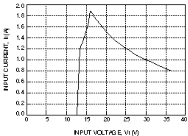
Figure 1. CC025 Triple-Output-Series Typical Input Characteristics
